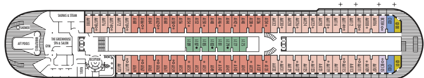
UPPER PROMENADE DECK Staterooms 100-189
