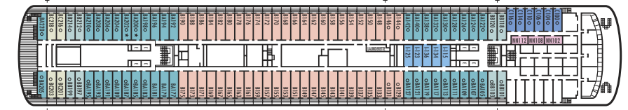
VERANDAH DECK Staterooms 100-220
