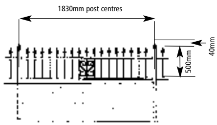
500mm high panel
