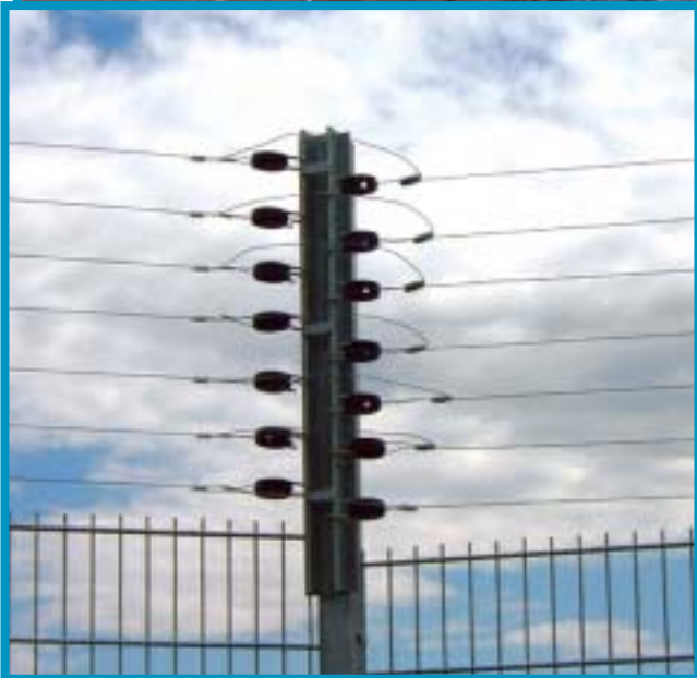
Alarm-aFence detail
