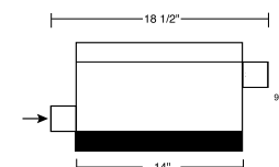
Diagram for part Numbers 21007HKR, 21008HKR
