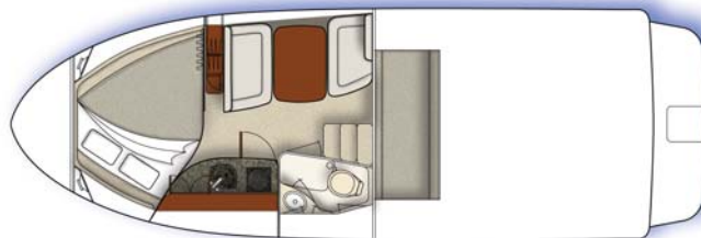
Cabin Layout
