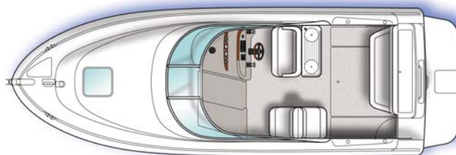
Cockpit Layout w/Standard Seating (Shown w/Optional Bait Prep Station)
