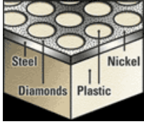
CONSTRUCTION OF DMT®'s INTERRUPTED SURFACE
