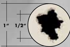
Typical Target 1416: 10-shot .22 l.r. test fire group at 55 yards.
