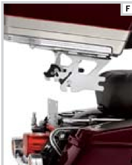
F. DETACHABLE TOUR-PAK MOUNTING RACK KIT FOR ELECTRA GLIDE CLASSIC MODELS – '97-'08 MODELS
