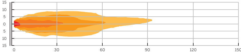
Original Equipment – Halogen Headlamps With Reflector Optics (7") Birds Eye View, (shown in feet)
