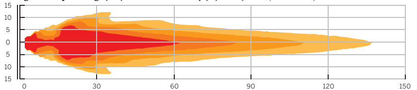
A. HIGH INTENSITY DISCHARGE (HID) DUAL BULB HEADLAMP KIT – ELECTRA GLIDE SHOWN
