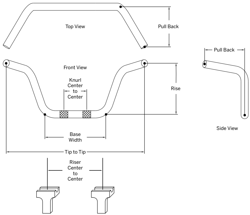
Handlebar Measurements
