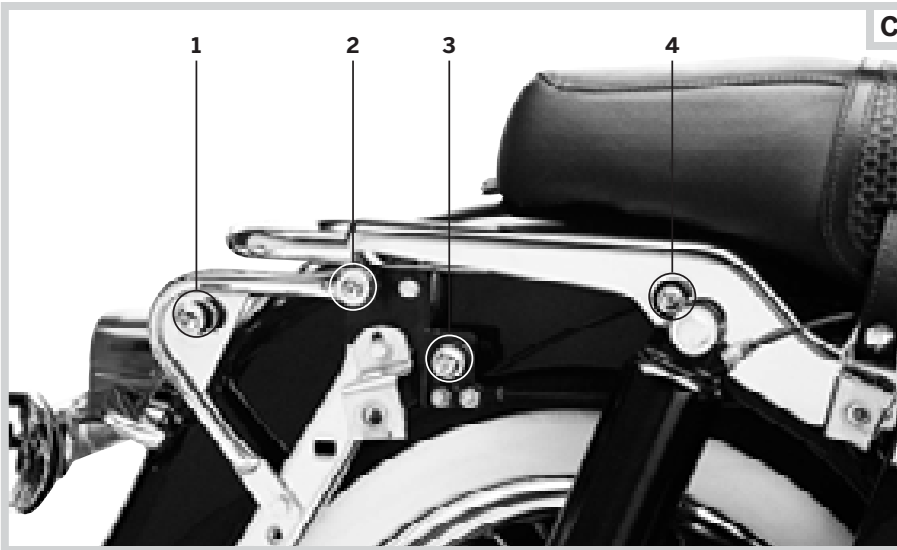
C. DETACHABLE DOCKING HARDWARE KIT – '97-'08 TOURING MODELS
