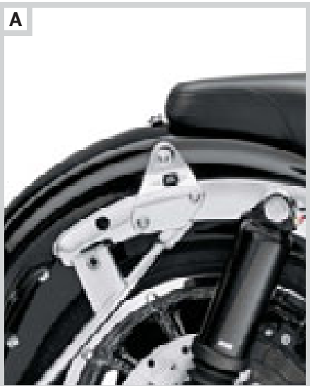
A. 2-POINT DOCKING HARDWARE KIT – CHROME
