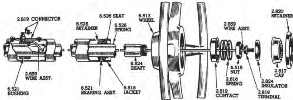
HORN CONTACT PARTS—CAB-OVER-ENGINE
