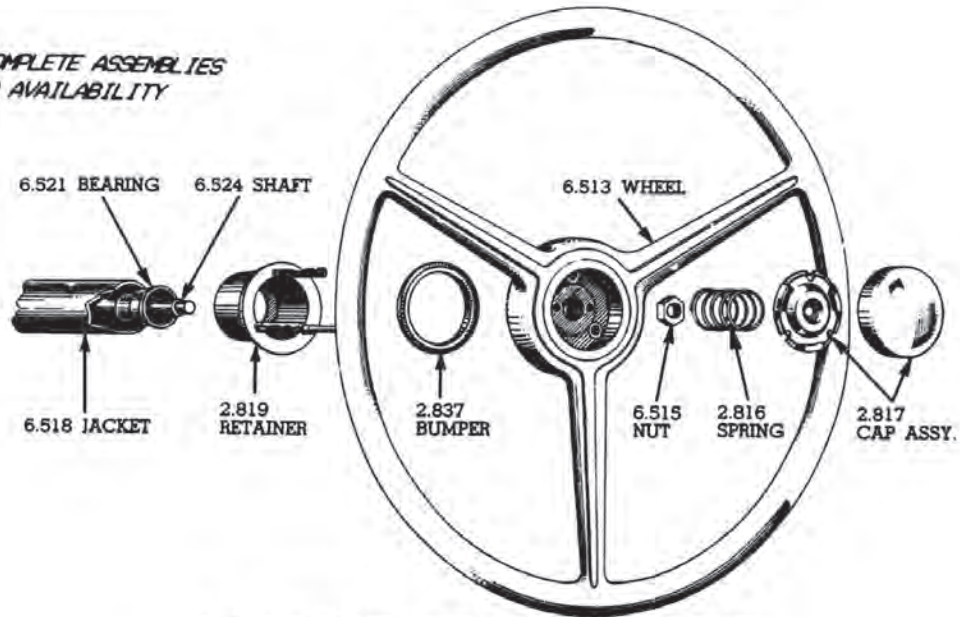
HORN CONTACT PARTS—CONVENTIONAL TRUCK
