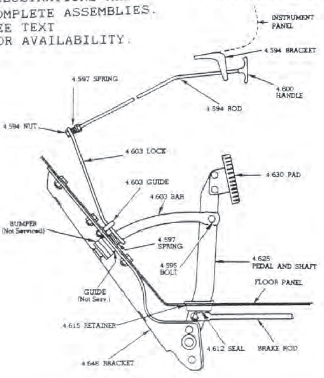
TRUCK PARKING BRAKE CONTROLS (FOOT OPER.)
