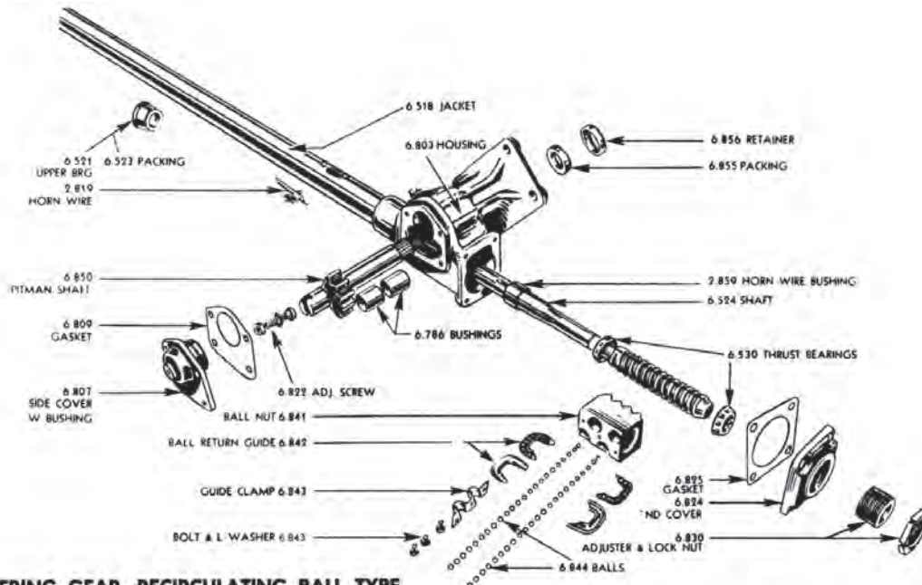
1941-46 STEERING GEAR—RECIRCULATING BALL TYPE
