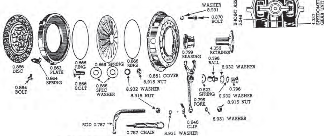
DIAPHRAGM SPRING BOLTED TYPE CLUTCH PARTS
