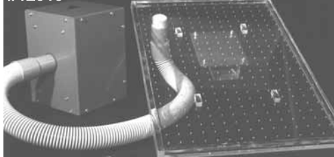
VACUUM PLATEN, MOTOR & FOOT SWITCH
