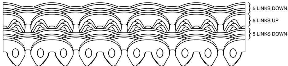
Typical Duplex Chain Assembly - RPDUP404 - 5-5-5 Assembly
