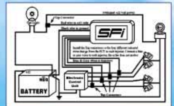
All Stock Fuel SFi Turned Off
